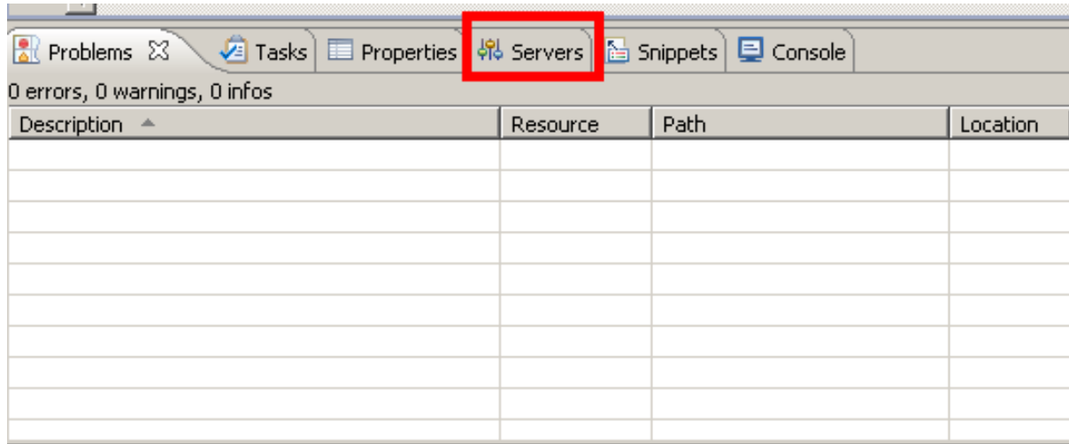
Figure 2.8. Launching Tomcat
