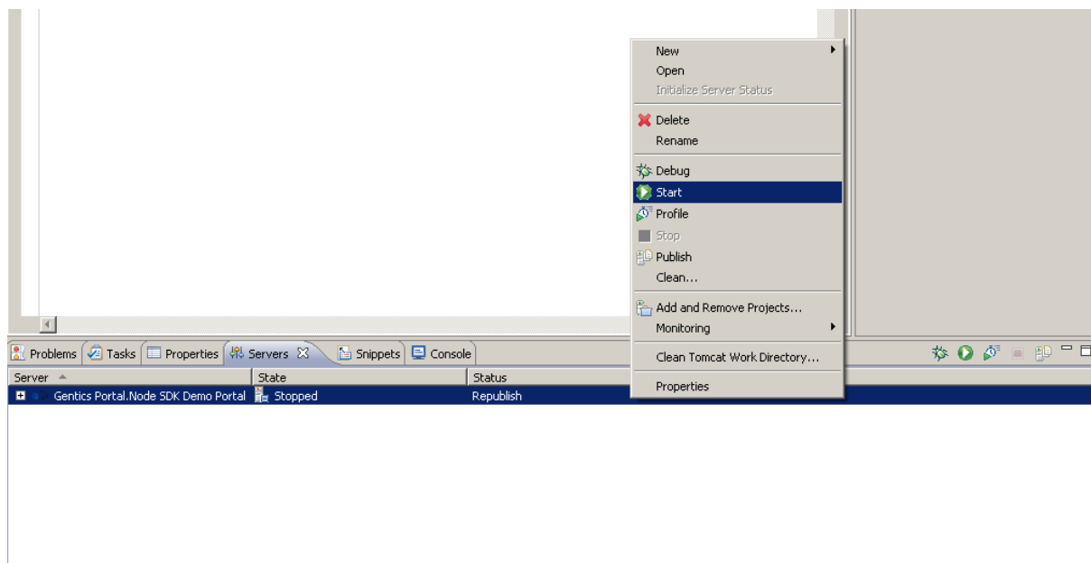
Figure 2.9. Launching Tomcat
